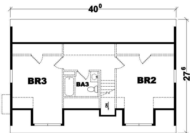
Proposed Second Floor Layout
