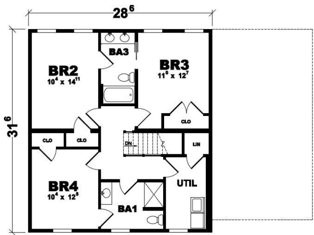
Second Floor Layout
