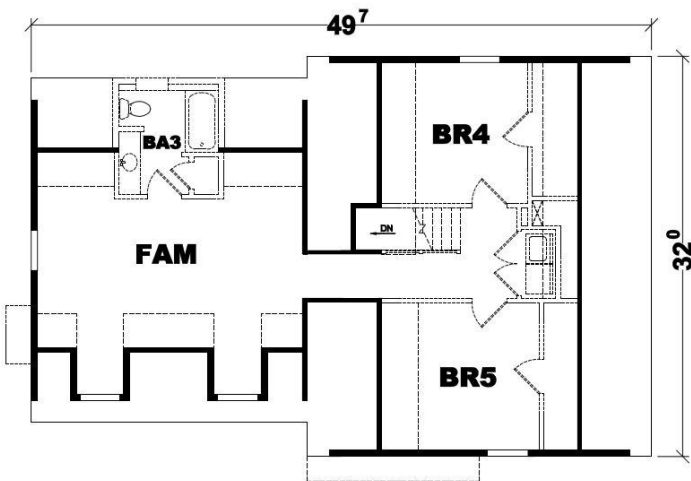
Proposed Second Floor Layout
